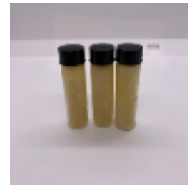
Cannabinoids (% weight)
